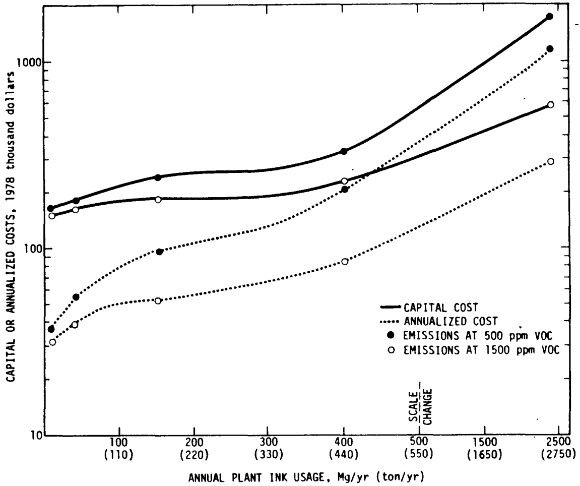
Figure 4-2. Capital and annualized costs of thermal incinerator with 50% primary heat recovery for VOC control at existing graphic arts plant using flexographic and rotogravure printing process for packaging.
