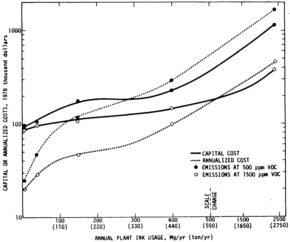
Figure 4-1. Capital and annualized costs of thermal incinerator without heat recovery for VOC control at existing graphic arts plant using flexographic and rotogravure printing process for packaging.
